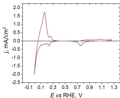
Fig. 2. Chronovoltamperometric curves recorded for a thin layer of palladium deposited on a gold substrate in 0.5 M H_2SO_4 ; scan rate v = 10 mV/s
