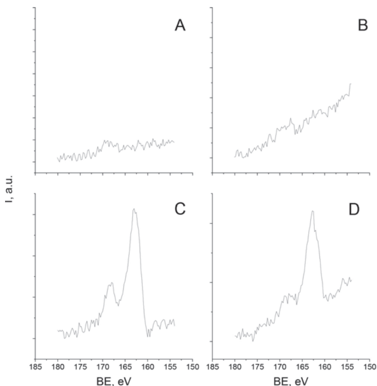
Fig. 8. XPS spectra in the S 2p range for Pd samples with small and large surface area, before and after being placed in the hydrocarbon stream; A – reference sample with small surface area, B – reference sample with large surface area, C – sample with low surface area after placing the electrode in the stream of hydrocarbons, D – sample with high surface area after placing the electrode in the stream of hydrocarbons
