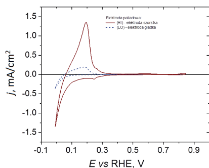
Fig. 4. Chronovoltamperometric curves recorded in the potential range of 0.0–0.845 V vs. RHE for palladium electrodes with a high (HI) and low (LO) degree of surface development in 0.5 M H_2SO_4 ; scan rate v = 10 mV/s
