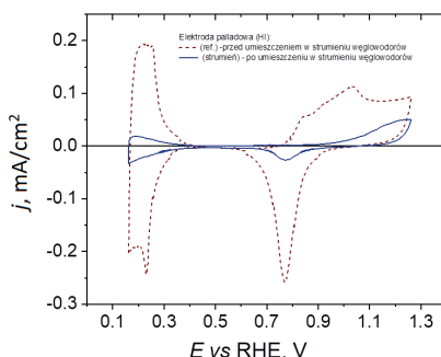
Fig. 5. Chronovoltamperometric curves recorded for the electrode (HI) before (ref.) and after (stream) placing it in the stream of hydrocarbons; scan rate v = 10 mV/s in 0.5 M H_2SO_4
