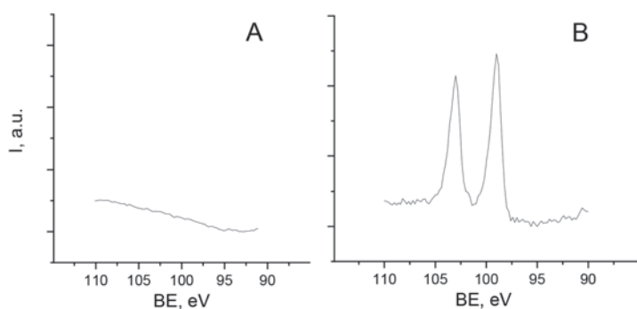
Fig. 10. XPS spectra in the Hg 4f range for Pd samples with small and large surface area, before and after being placed in the hydrocarbon stream; A - reference sample with a small surface area, B - reference sample with a large surface area (HI) stream (14 days)
