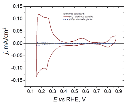
Fig. 3. Chronovoltamperometric curves recorded in the potential range of 0.15–0.875 V vs. RHE for palladium electrodes with a high (HI) and low (LO) degree of surface development in 0.5 M H_2SO_4 ; scan rate v = 10 mV/s
